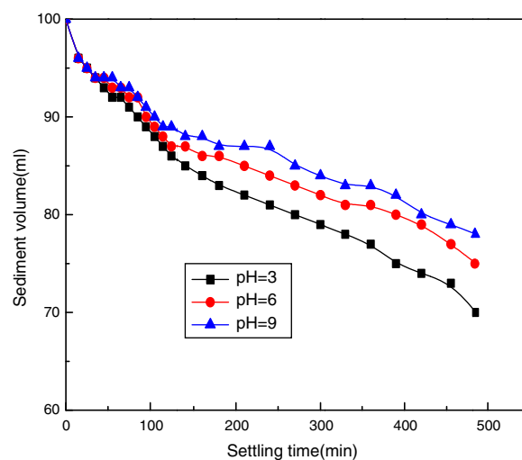
Fig. 2 – Effect of pH on the settling behavior of quartz.
