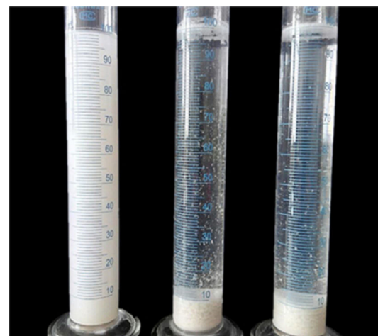
Fig. 5 – Effect of chitosan on the settling behavior of quartz at different pH (settling time = 5 min; left: pH = 3, middle and right: pH = 9).
