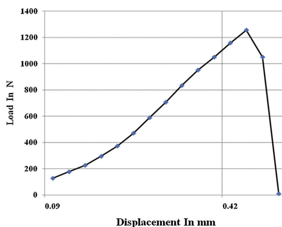
Fig. 6 – Loading Curve of SG cast iron.
