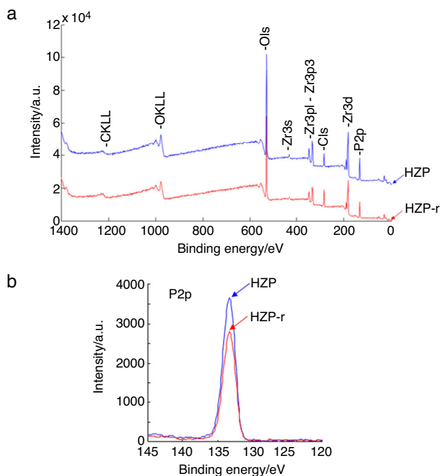
Fig. 2 – XPS wide spectra (a) and P2p XPS spectra (b) of HZP and HZP-r.
