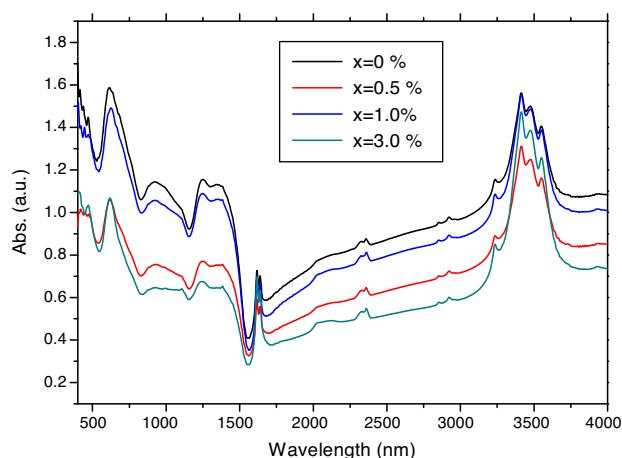
Fig. 2 – FTIR for base glass and glass doped with x mol% Eu 2 O 3 .
