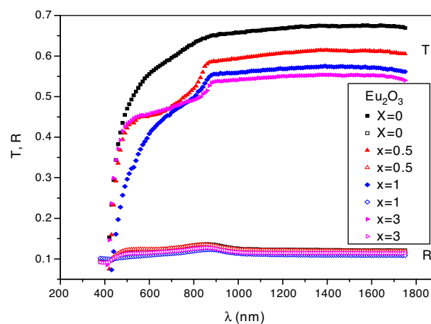
Fig. 3 – The transmittance T(λ) and the reflectance R(λ) spectra for ZnO boro-tellurite glasses doped with x Eu 2 O 3 .
