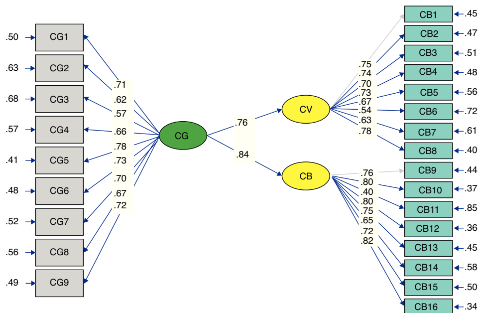
Figure 2. Graphical Solution of the Structural Equations Model.
