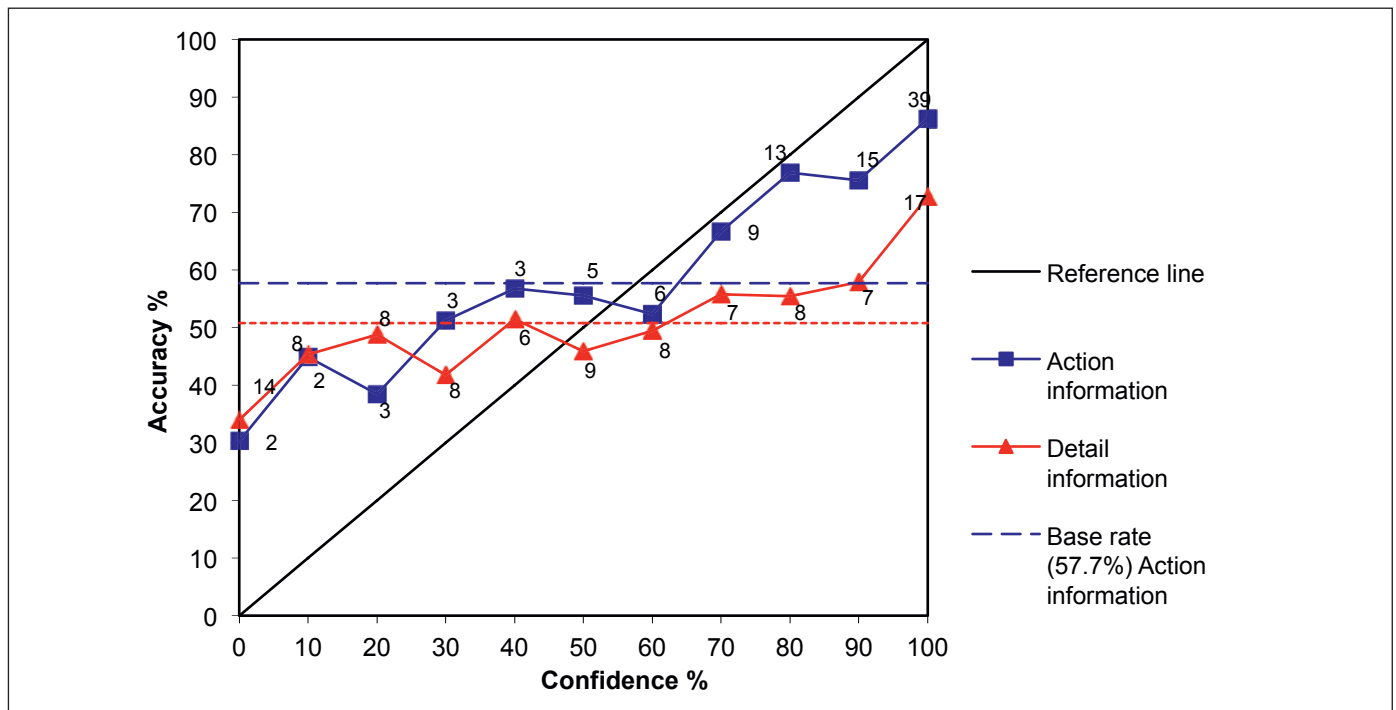
Figure 2. Experiment 2: Calibration curves for the focused questions for action and detail information. Digits at each point show the % of confidence judgments that used this confidence level at that particular level of proportion correct. 0 % on the confidence axis (x) means “Completely sure that I remember wrong” and 100 % means “Completely sure that I remember correct”.
