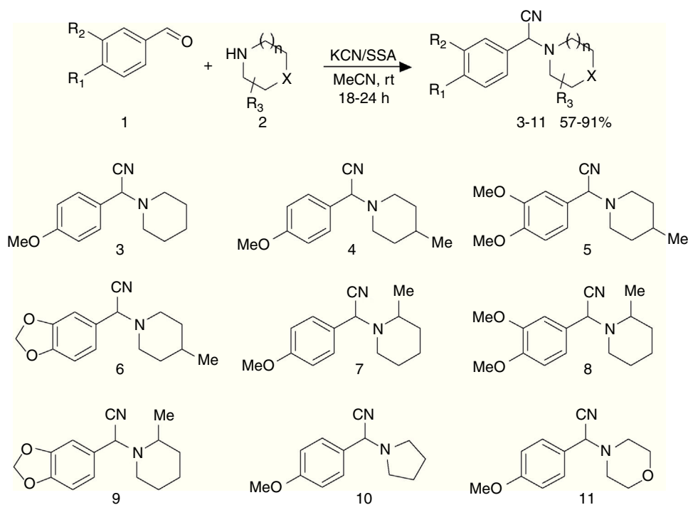
Scheme 1. Preparation of new \alpha -amino nitriles 3–11 by modified Strecker reaction.
